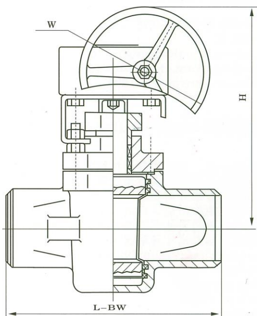
L-BW (Gear Operated)
