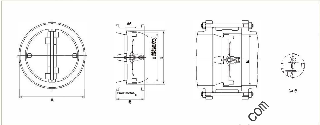
Wafer type
