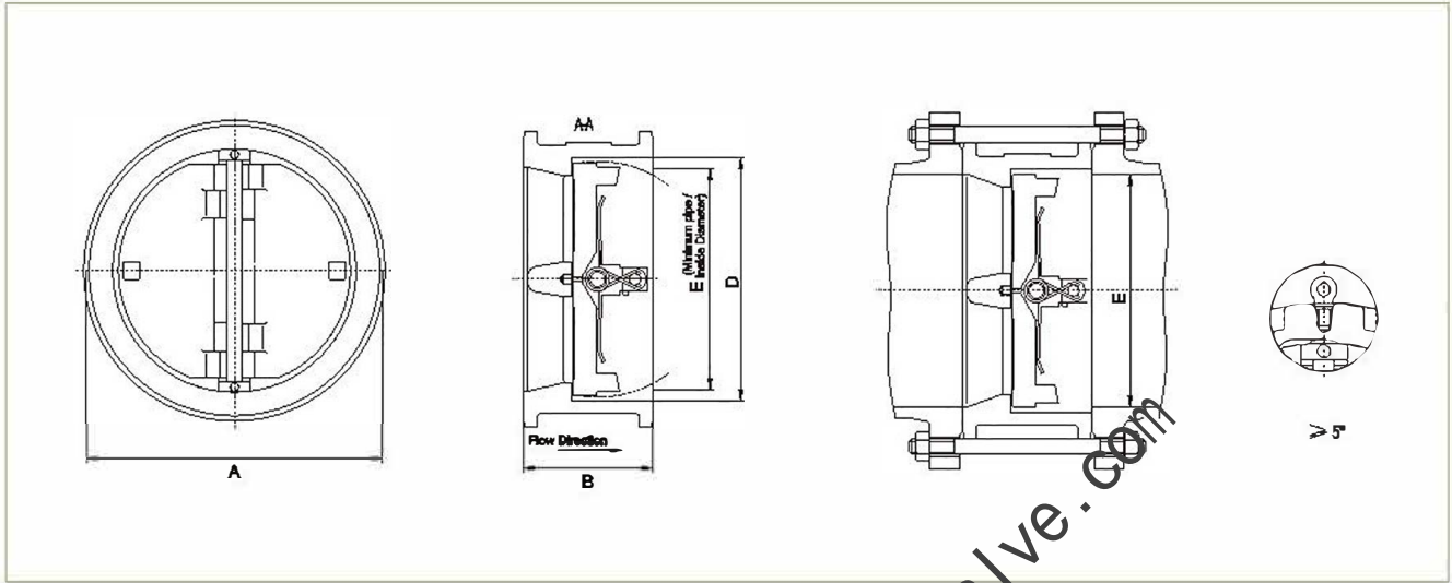
Wafer type
