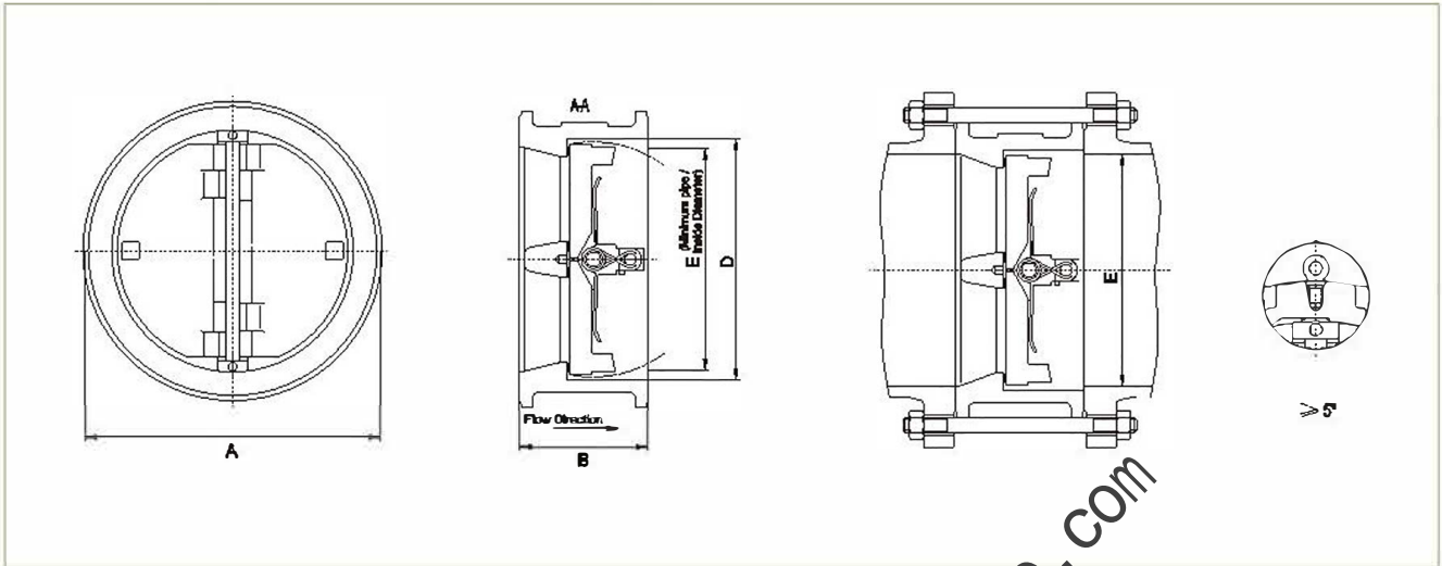
Wafer type
